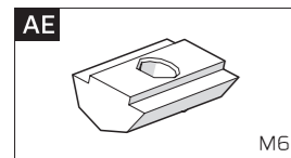
Ball Bearing Nut NS-M6 X12
